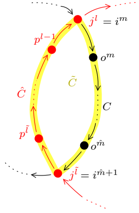
Figure 3: Construction of \tilde{C} for Case 2 in the proof of Lemma 8.
