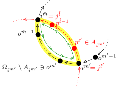
(a) As described in Case 4.1 in the proof of Claim 7, the highlighted path forms a CIC of \mu + C at A for i^{m'} , the agent with highest priority for whom the statement of the claim is violated. Notice that since this is a CIC of \mu + C , we use a section of C in reverse—that is, we undo some of what C does.
